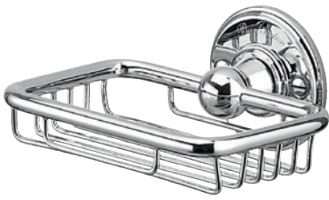
Soap basket W 140 | D 120 | H 60
